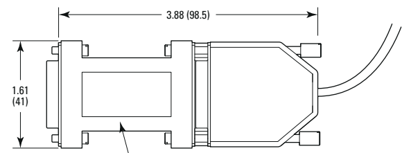
ENCODER 3 x SUB-D15M CONNECTOR, CABLE LENGTH 9.8 FT (3 M)
