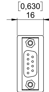
Mating connector: Male SubD9 with UNC4/40 lockers
